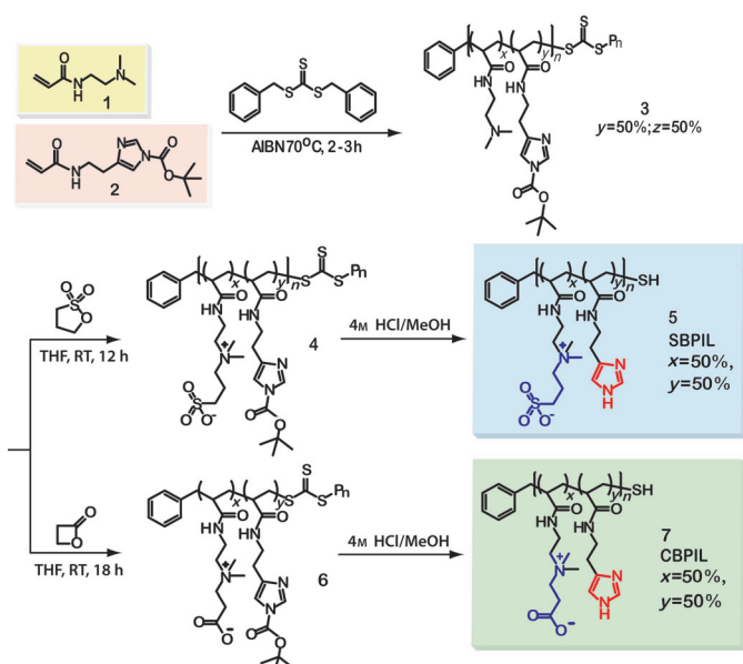
Scheme 1. Scheme for synthesis of sulfobetaine- and carboxybetaine-functionalized poly(imidazole) ligands (SBPILs and CBPILs). Random copolymer backbones (3) are synthesized through radical addition fragmentation chain transfer (RAFT)-mediated polymerization and betainized using 1,3-propanesultone and \beta -propiolactone to yield SBPILs (5) and CBPILs (7), respectively. AIBN = azobisisobutyronitrile.
